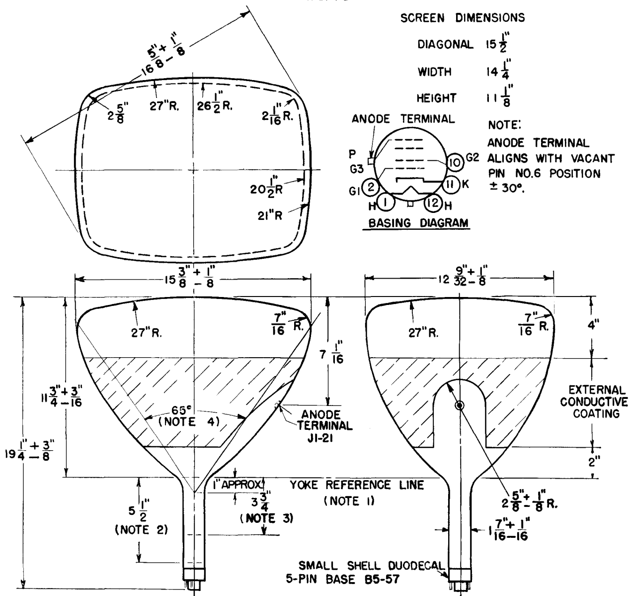
OUTLINE 17BP4-B
