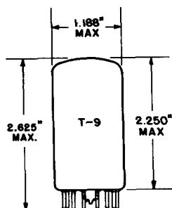
GLASS BULB BUTTON 12 PIN BASE E12-70
