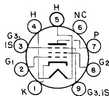
BOTTOM VIEW BASING DIAGRAM JEDEC 96K
