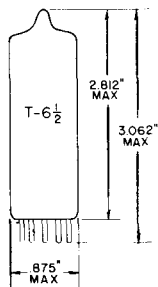
GLASS BULB MINIATURE BUTTON 9 PIN BASE E9-1 OUTLINE DRAWING JEDEC 6-4
