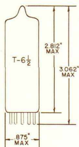
GLASS BULB
