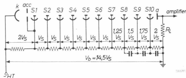
voltage divider type B 1)
