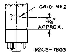
Fig. 2 - Location of Grid No. 2 in Tube Neck.
