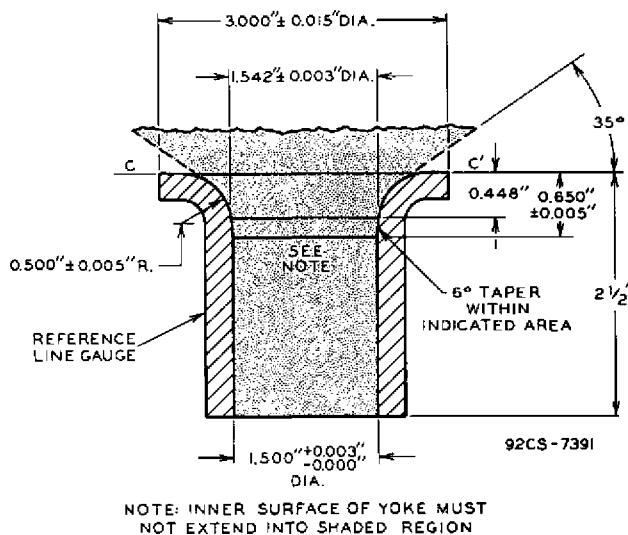
Fig. 2 - Reference-Line Gauge (JETEC No. 110) with Supplementary Information on Recommended Inside Contour of Yoke to Provide Proper Location of Yoke on Neck-Funnel Section.
