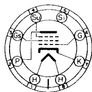
8V BOTTOM VIEW
