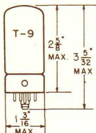
GLASS BULB
