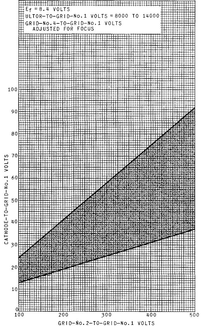
Fig. 3 - Raster-Cutoff Range for Type 14ATP 4 in Cathode-Drive Service.
