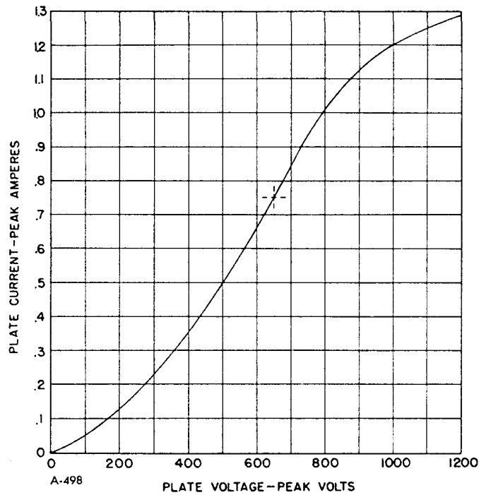
PLATE CURRENT CHARACTERISTICS
