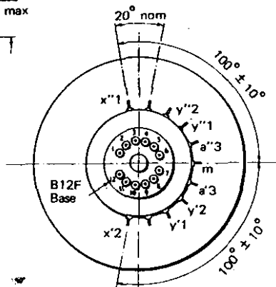
View in direction of arrow A
