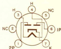
BOTTOM VIEW BASING DIAGRAM JEDEC 5BS
