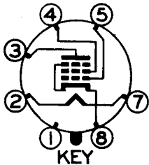
RETMA 7AC BOTTOM VIEW
