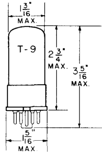
GLASS BULB
