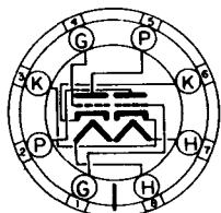
BOTTOM VIEW INTERMEDIATE SHELL 8 PIN OCTAL
