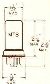
6SK7 METAL SHELL
