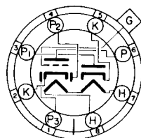
BOTTOM VIEW INTERMEDIATE SHELL 8 PIN OCTAL BASE 8C9
