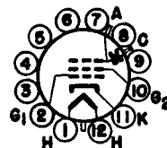
BASING DIAGRAM 12N
