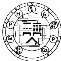
BOTTOM VIEW MINIATURE BOTTOM 9 PIN BASE
