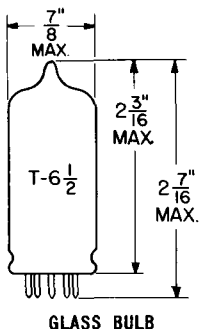
GLASS BULB
