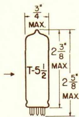
GLASS BULB MINIATURE BUTTON 9 PIN BASE B9-1 OUTLINE DRAWING JEDEC 6-3
