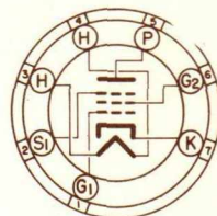
BOTTOM VIEW MINIATURE BUTTON 7 PIN BASE 7BK
