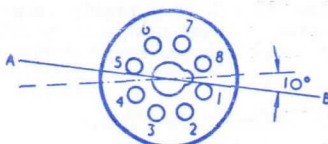
Viewed from free end of pins
