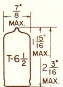
GLASS BULB
