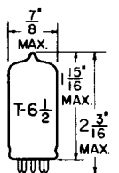
GLASS BULB
