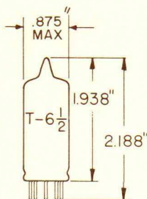
GLASS BULB MINIATURE BUTTON 9 PIN BASE E9-1
