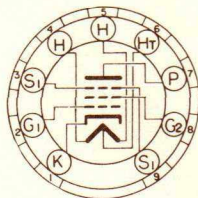
BOTTOM VIEW SMALL BUTTON 9 PIN BASE 9BF
