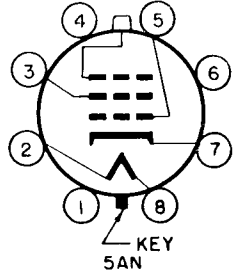
BOTTOM VIEW OF BASE
