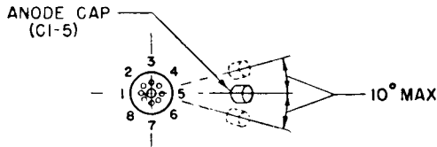
BOTTOM VIEW OF TUBE
