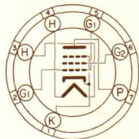
BOTTOM VIEW MINIATURE BUTTON 7 PIN BASE 7CV
