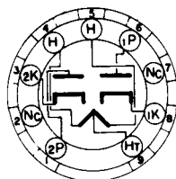
BOTTOM VIEW MINIATURE BUTTON 9 PIN BASE 985
