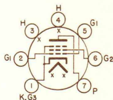
BOTTOM VIEW BASING DIAGRAM JEDEC 7CV
