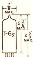
GLASS BULB
