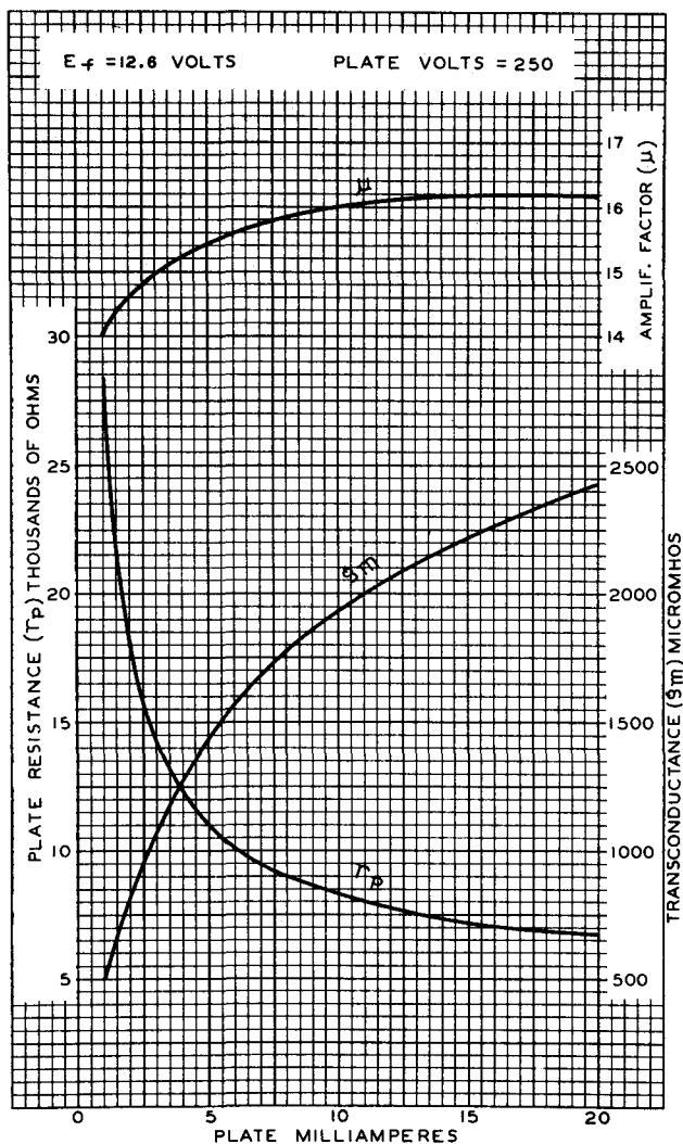
Fig. 2 - Average Characteristics for Triode Unit of Type 12BF6.
