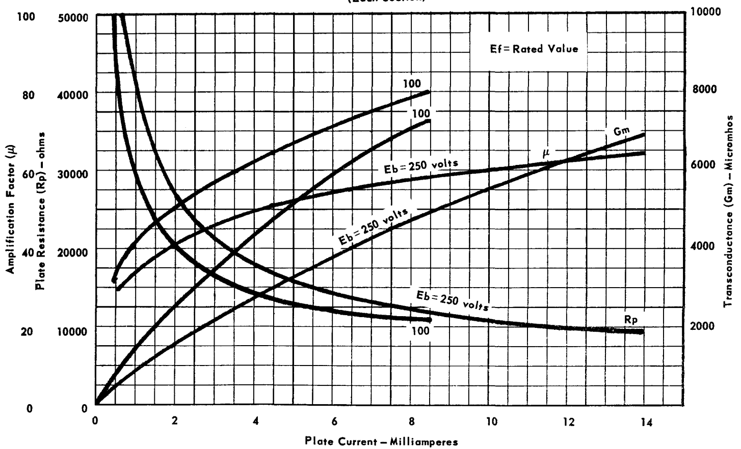
AVERAGE CHARACTERISTICS (Each Section)
