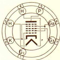
BOTTOM VIEW MINIATURE BUTTON 7 PIN BASE TCH
