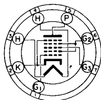
BOTTOM VIEW MINIATURE BUTTON 7 PIN BASE 7CH
