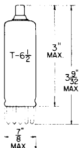
GLASS BULB
