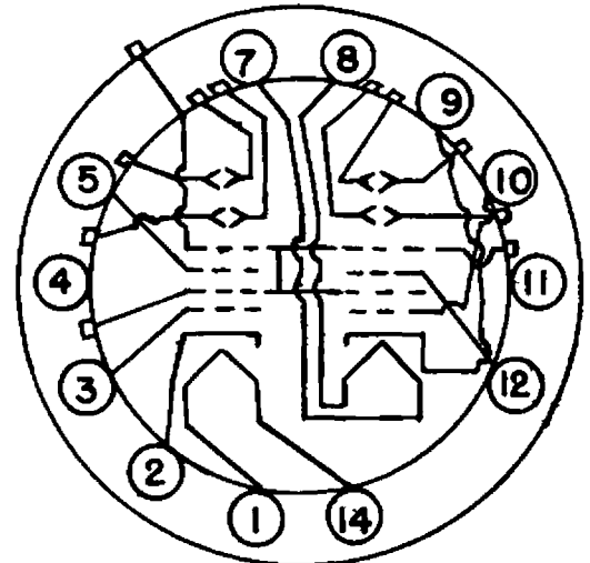
BASING DIAGRAM
