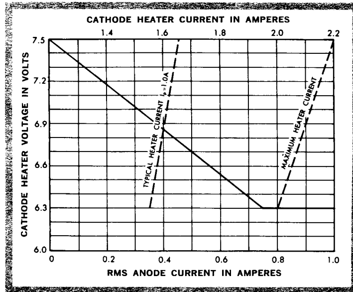
RECOMMENDED HEATER VOLTAGE CURVE
