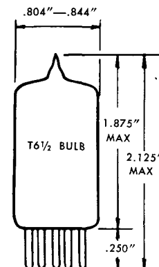
OUTLINE DRAWING
