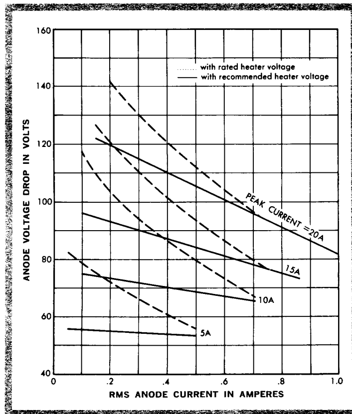
TYPICAL ANODE VOLTAGE DROP CURVE
