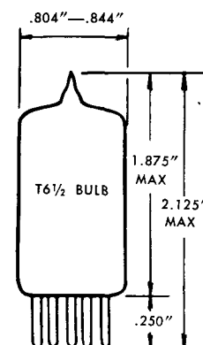
OUTLINE DRAWING
