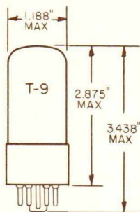
GLASS BULB INTERMEDIATE SHELL 8 PIN OCTAL BB-6 OUTLINE DRAWING JEDEC 9-15
