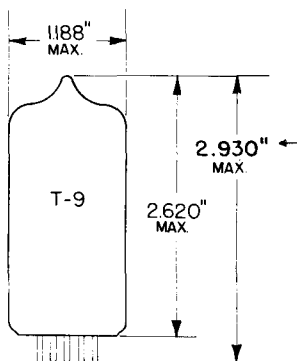
GLASS BULB BASE E9-68 JEDEC OUTLINE 9-70
