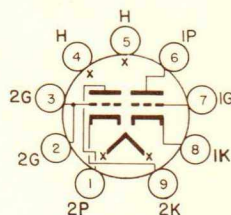
BOTTOM VIEW BASING DIAGRAM JEDEC 9HF
