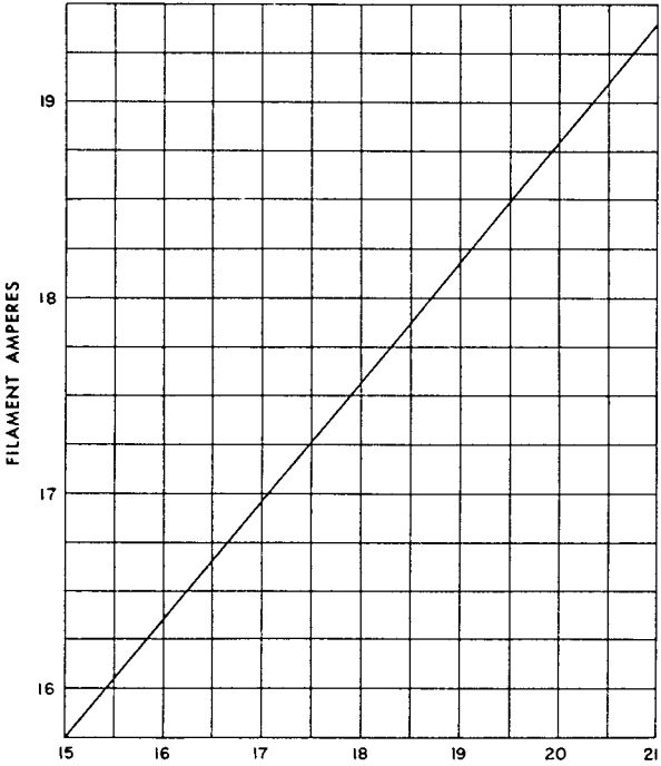
FILAMENT CHARACTERISTICS A-8473
