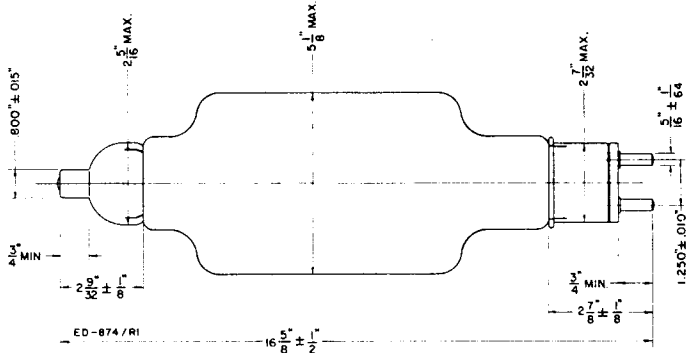
DIMENSIONS—ML-102A
