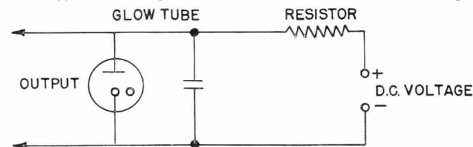
Fig. 2—Relaxation Oscillator Circuit 9-25-44
