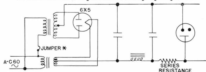
Fig. 1—Voltage-Regulated Power Supply Circuit 9-25-44
