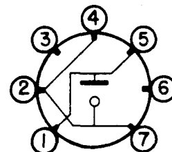
BOTTOM VIEW 580
