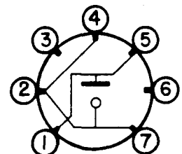
BOTTOM VIEW 580
