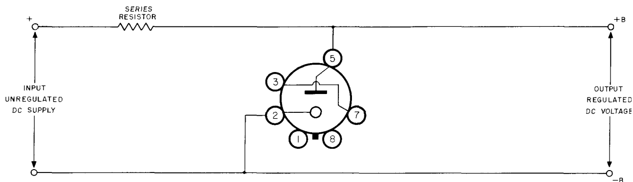
FIG. 1 — BASIC REGULATOR CIRCUIT
