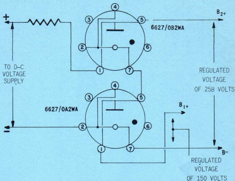
OPERATION OF REGULATOR TUBES IN SERIES
