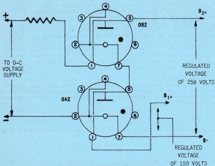
OPERATION OF REGULATOR TUBES IN SERIES
