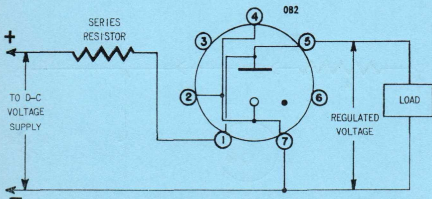
TYPICAL CIRCUIT FOR VOLTAGE REGULATOR
